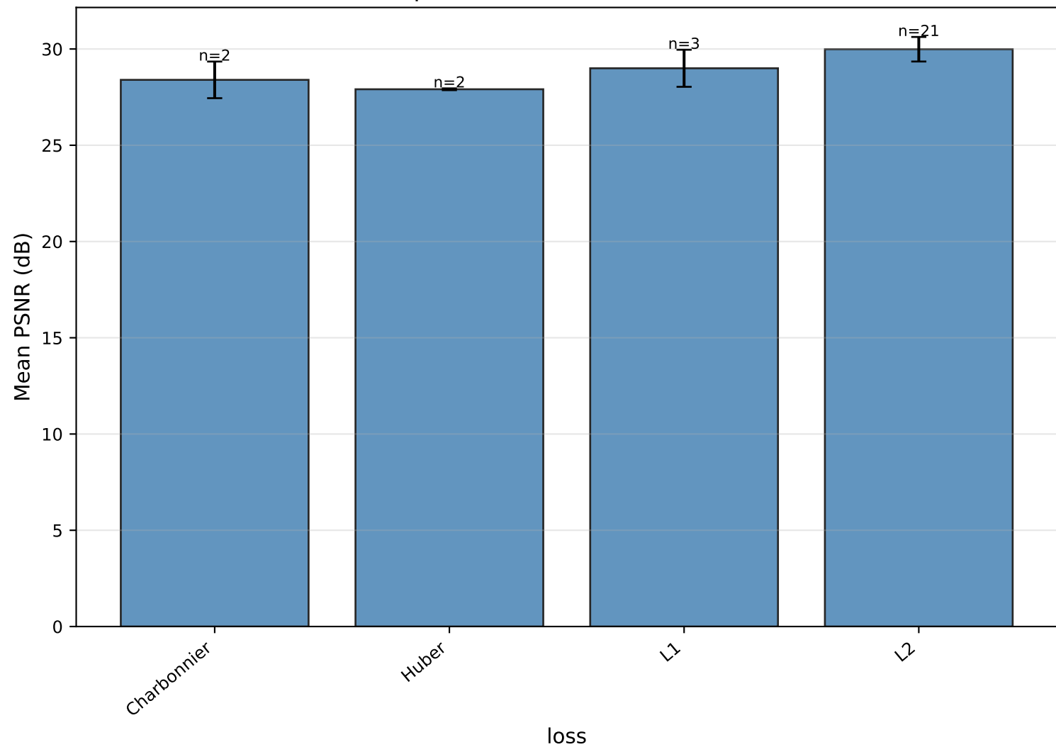
Mean PSNR per value of loss — WaveletAttention
